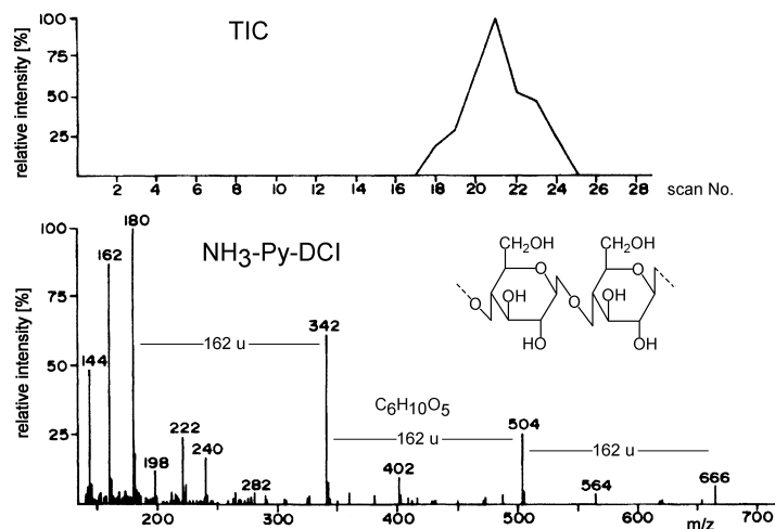
Fig. 7.15. Ammonia-Py-DCI mass spectrum of cellulose and total ion current. Adapted from Ref. [91] by permission. © Research Council of Canada, 1994.
