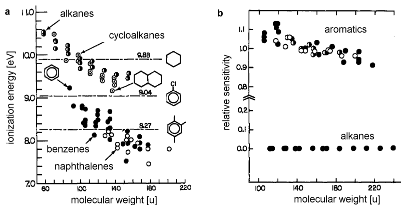
Fig. 7.10. (a) Ionization energies of certain classes of organic molecules as a function of their molecular weight, and (b) relative sensitivities for (○) alkylbenzenes, (●) polyolefines, and (◐) substituted naphthalenes in chlorobenzene CE-CI. Adapted from Ref. [51] by permission. © American Chemical Society, 1983.
