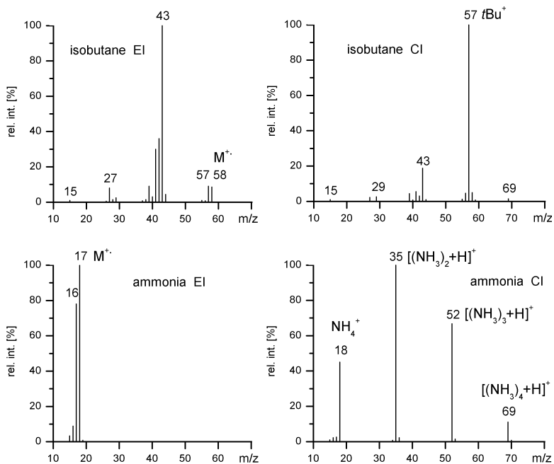
Fig. 7.6. Standard EI versus positive-ion CI spectra of isobutane (upper) and ammonia (lower part). Ammonia forms abundant cluster ions upon CI.
